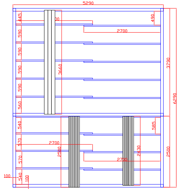
Foundation and floor joist plan
